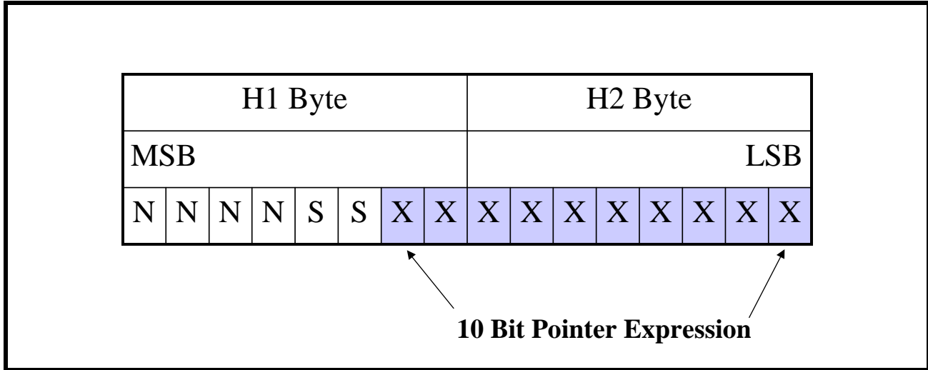
Figure 50 relates the contents within these 10 bits (within the H1 and H2 bytes) to the location of the J1 byte (e.g., the very first byte of the STS-1 SPE) within the Envelope Capacity.
