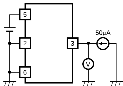
Test Circuit 4
