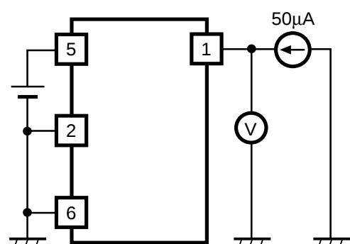
Test Circuit 6
