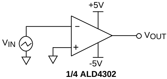
ZERO CROSSING DETECTOR
