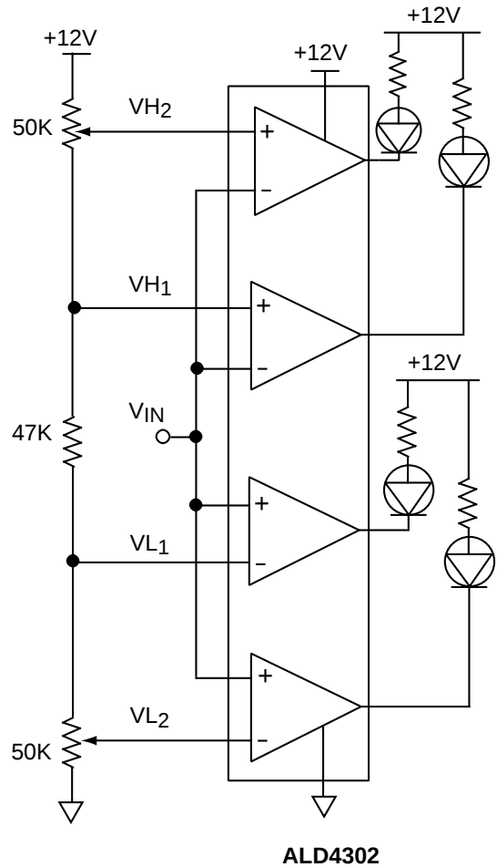
DOUBLE DUAL LIMIT WINDOW COMPARATOR
