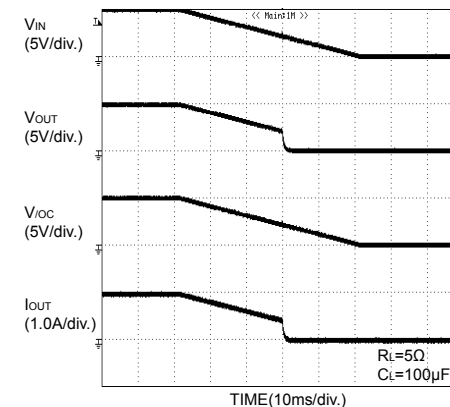
Fig.38 UVLO response decreasing V IN
