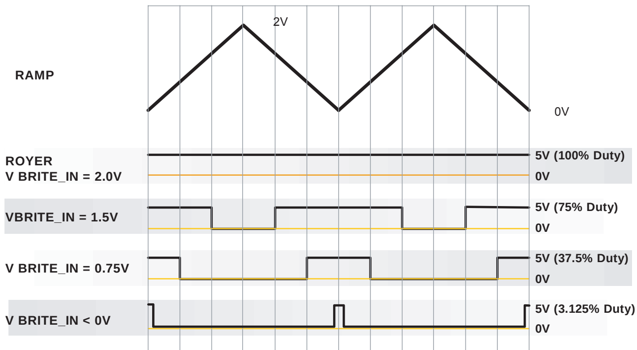
Figure 3 – Timing Diagram
