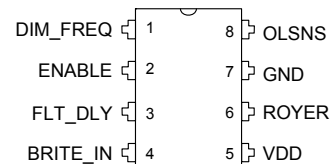
M Package (Top View)
