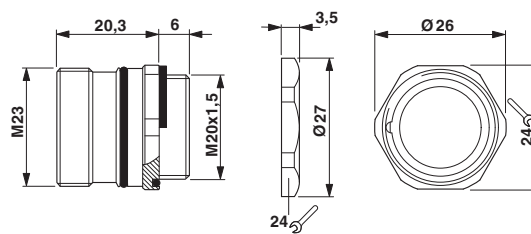
Dimensioned drawing
