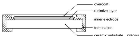
Fig. 3 Chip resistor outlines
