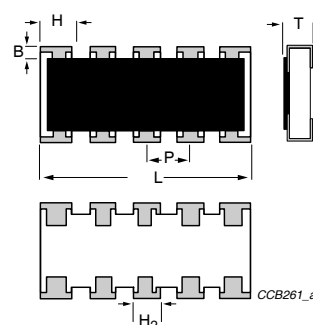
Fig. 4 YC124 series chip resistors dimension
