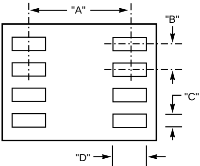
Concave and Convex Chip Resistor Arrays 742-746
