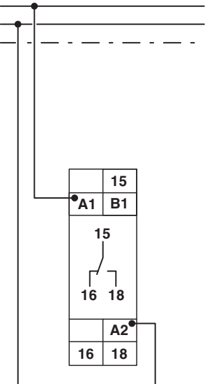
Figure 2 Connection without control contact
