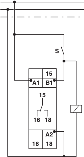
Figure 4 Connection with control contact and parallel load (e.g. relay)
