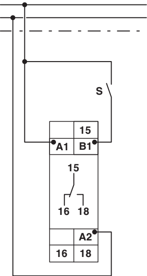
Figure 3 Connection with control contact
