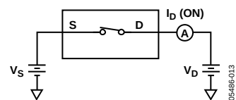
Figure 14. On Leakage
