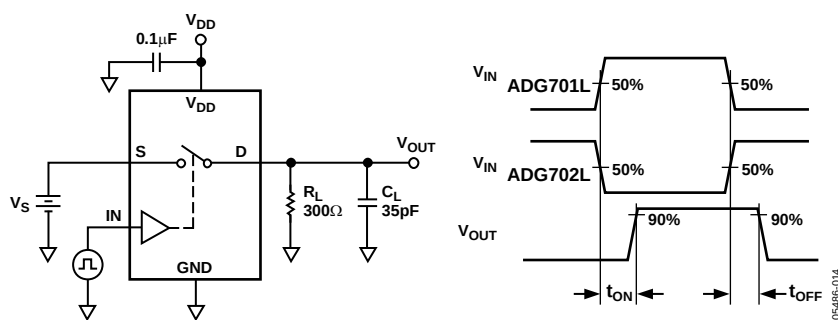
Figure 15. Switching Times
