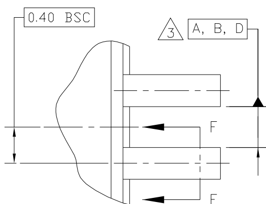
DETAIL G
