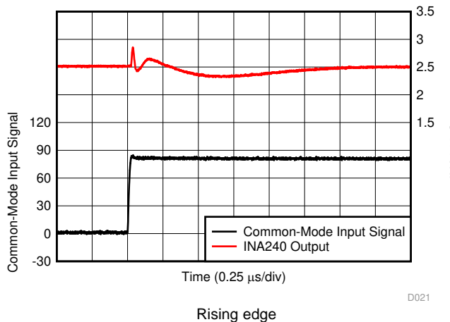
Figure 21. Common-Mode Voltage Transient Response
