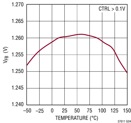
FB Regulation Voltage ( V_{\text{FB}} ) vs Temperature
