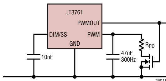
Figure 7. Configuration for Sub 4% PWM Dimming
