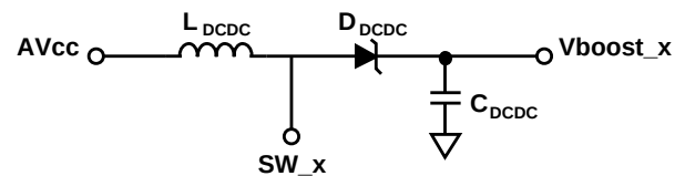
Figure 20. DC-DC Circuit
