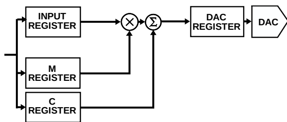
Figure 18. Digital Offset and Gain control
