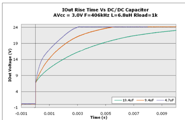
Figure 8. Iout settling 0-24mA through 1kΩ load, V_{CC}=3.0V , L_{DCDC}=10\mu H , DCDC frequency=406kHz, C_{DCDC} varied. (See Figure 20)
