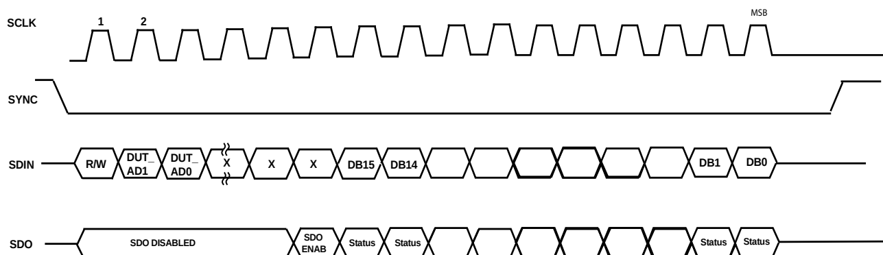
Figure 3. Readback Timing Diagram
