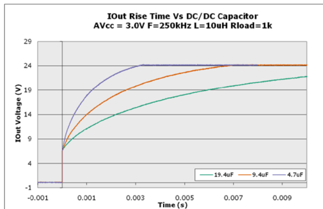
Figure 7. Iout settling 0-24mA through 1kΩ load, V_{CC}=3.0V , L_{DCDC}=10\mu H , DCDC frequency=250kHz, C_{DCDC} varied. (See Figure 20)
