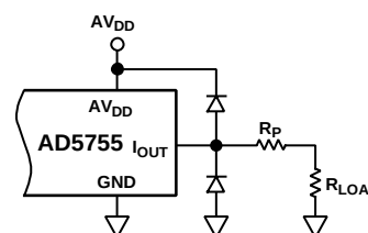
Figure 21. Output Transient Voltage Protection
