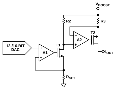
Figure 14. Voltage to Current conversion circuitry
