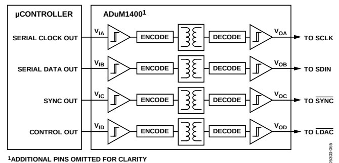
Figure 22. Isolated Interface
