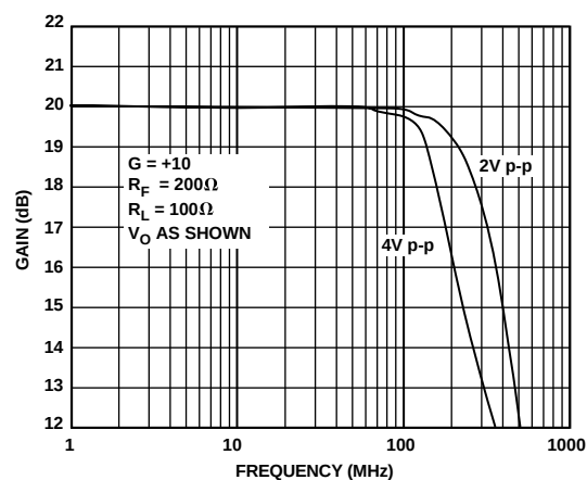
TPC 6. 大信号频率响应; G = +10
