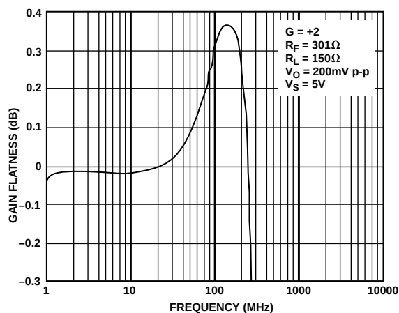
TPC 5. 增益平坦度; G = +2 ; V_S = 5\text{V}
