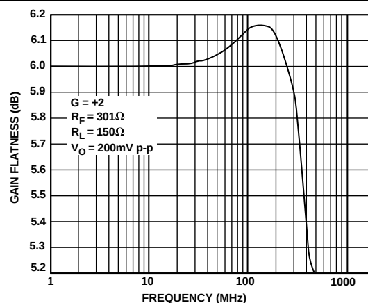
TPC 4. 增益平坦度; G = +2
