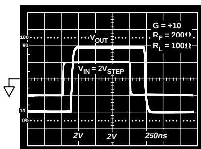
TPC 26. 过驱恢复; G = +10
