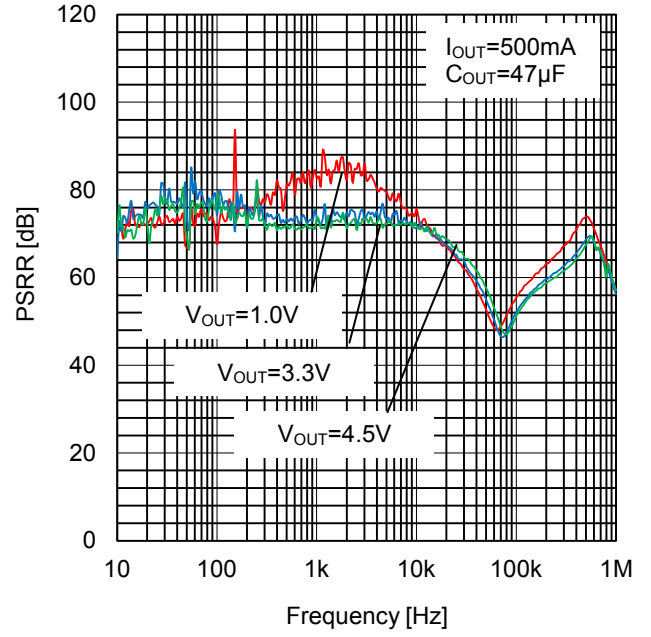
Figure 18. Power-Supply Rejection Ratio vs V_{OUT}
