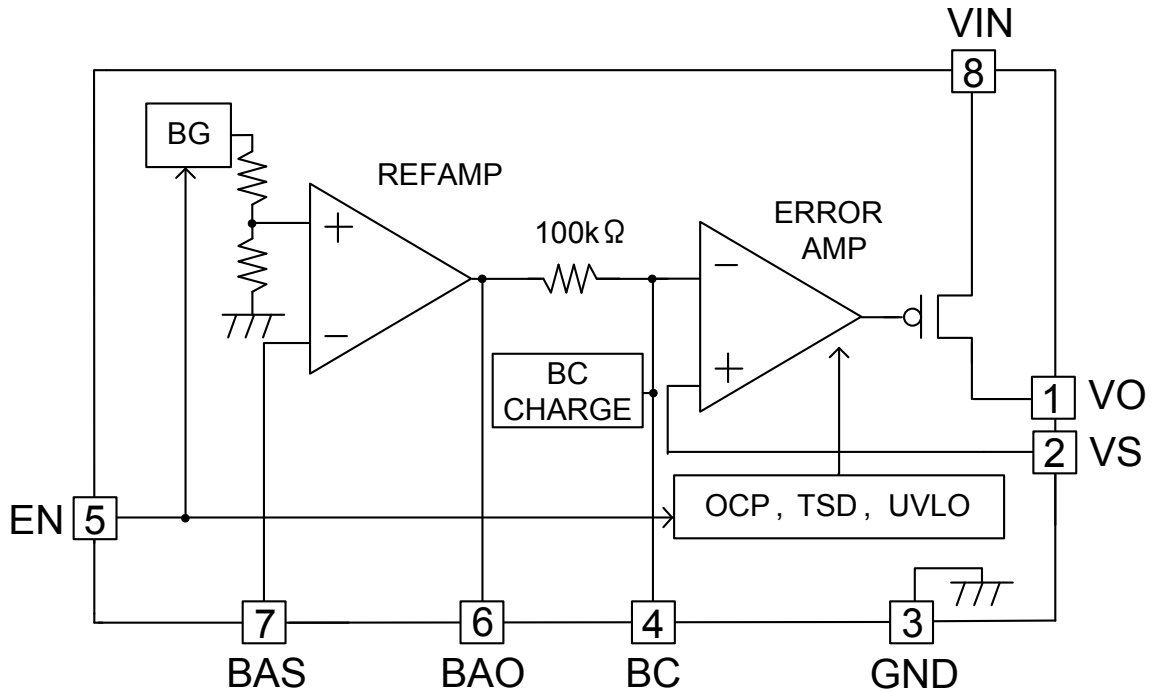
Figure 3. Block Diagram
