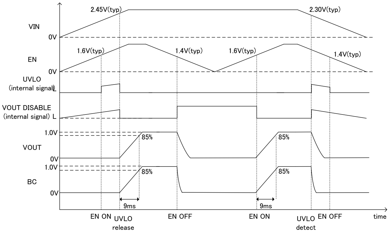
Figure 4. The Waveform During VIN/EN Rising and Falling (When at BC Capacitor 1 \mu F and Output 1V Settings)
