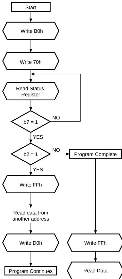
Figure 20. Program Suspend &amp; Resume Flowchart and Pseudo Code
