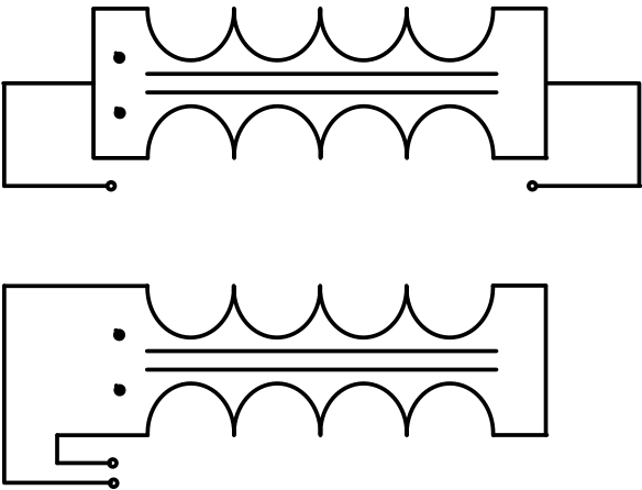
Differential Mode
