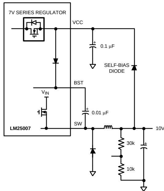
Figure 3. Self Biased Configuration
