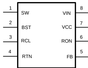
Figure 1. 8-Lead MSOP, LLP
