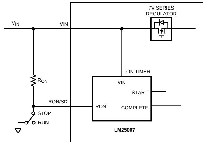
Figure 4. Shutdown Implementation
