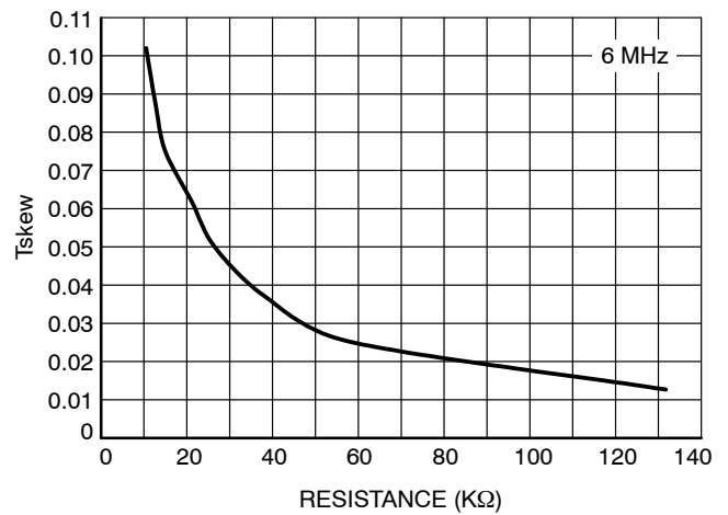
Figure 13. Tskew vs. Resistance (6 MHz, FS = 0)
