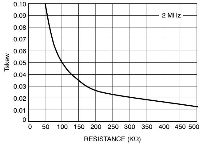
Figure 9. Tskew vs. Resistance (2 MHz, FS = 0)
