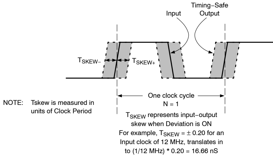
Figure 5. Input - Output Skew
