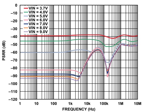
Figure 8. VOUT2 PSRR, I_{VOUT2} = 50\text{ mA}
