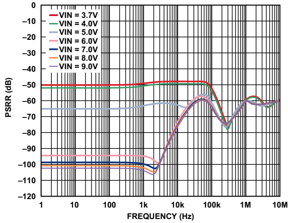
Figure 5. VOUT1 PSRR, I_{VOUT1} = 10\text{ mA}
