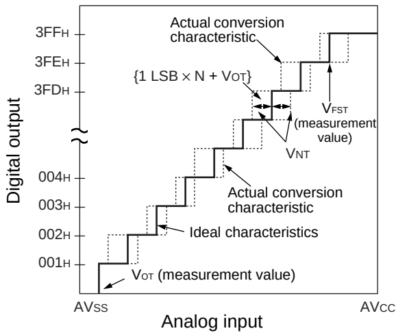
Linearity error
