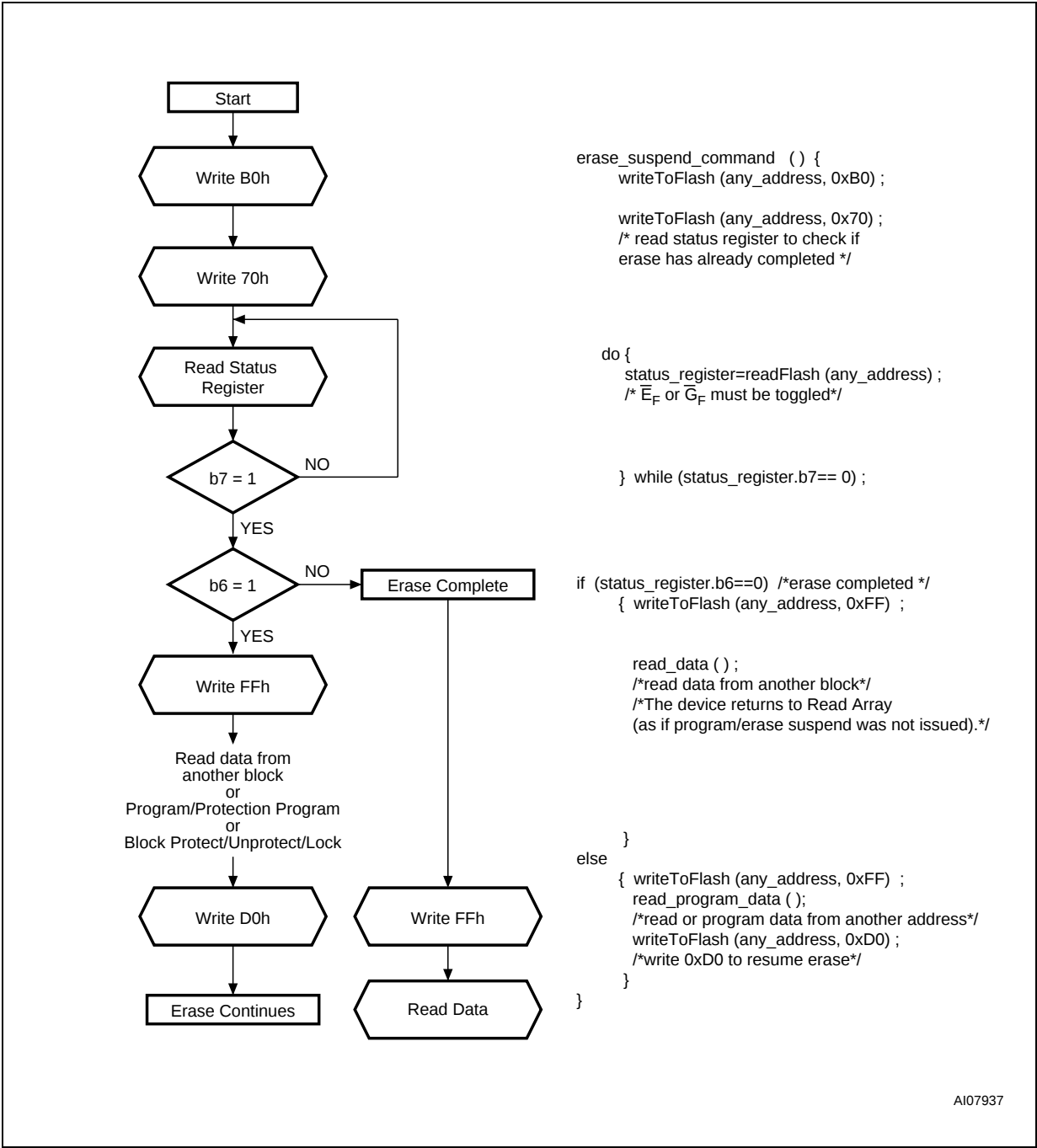
Figure 30. Erase Suspend & Resume Flowchart and Pseudo Code
