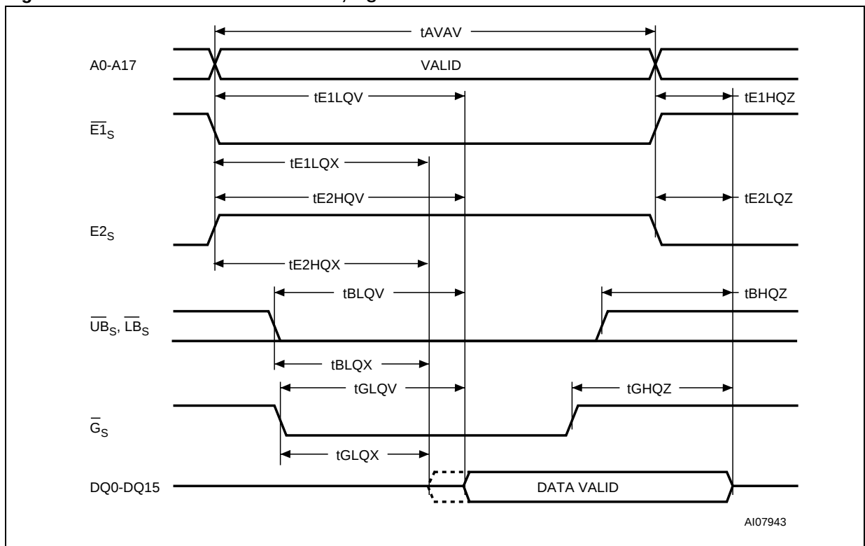
Figure 18. SRAM Read AC Waveforms, \overline{G}_S Controlled
