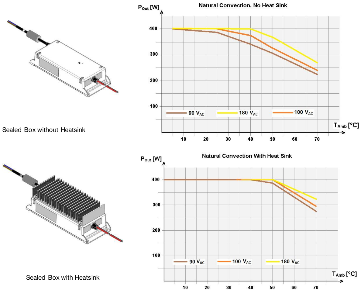
Figure 2. Power Derating Curves
