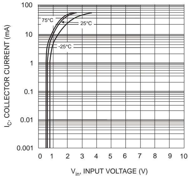
I_C , COLLECTOR CURRENT (mA) V_{in} , INPUT VOLTAGE (V) Fig. 5 Collector Current Vs. Input Voltage
