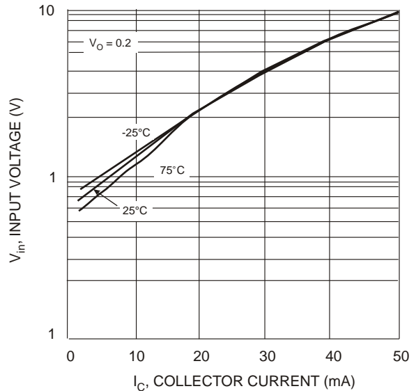
V_{in} , INPUT VOLTAGE (V) I_C , COLLECTOR CURRENT (mA) Fig. 6 Input Voltage vs. Collector Current
