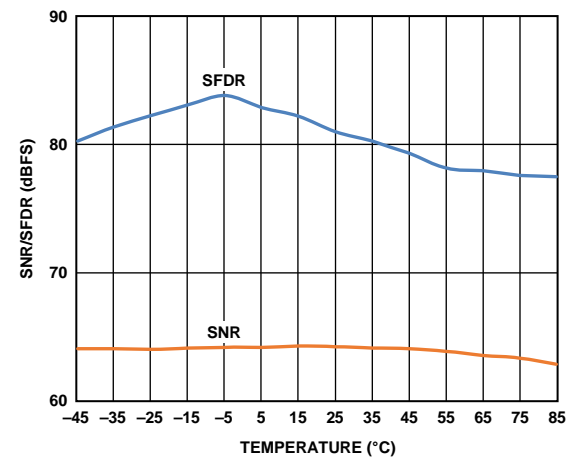
Figure 23. SNR/SFDR vs. Temperature, f_{IN} = 170.3 MHz
