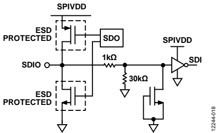
Figure 59. SDIO Input
