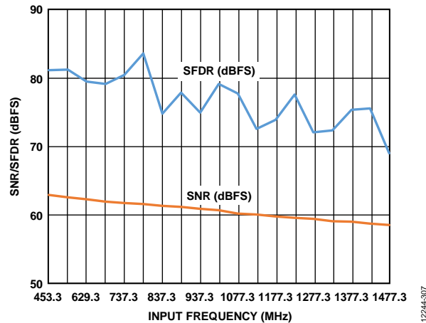
Figure 16. SNR/SFDR vs. Input Frequency ( f_{IN} ); 450 MHz < f_{IN} < 1500 MHz; Buffer Current = 7.5\times (Uses Circuit Shown in Figure 64)
