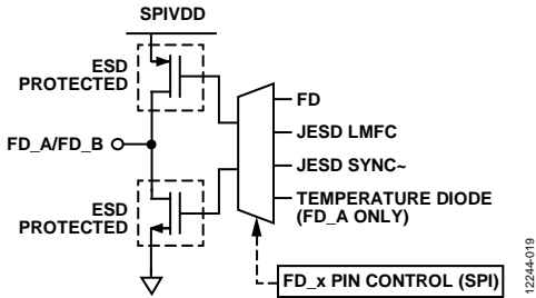
Figure 60. FD_A/FD_B Outputs
