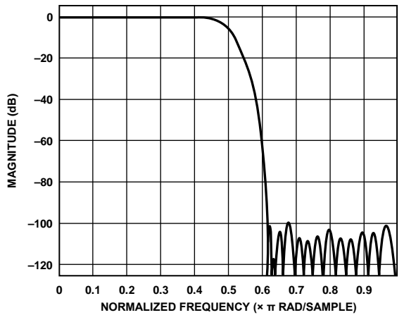
Figure 88. HB1 Filter Response
