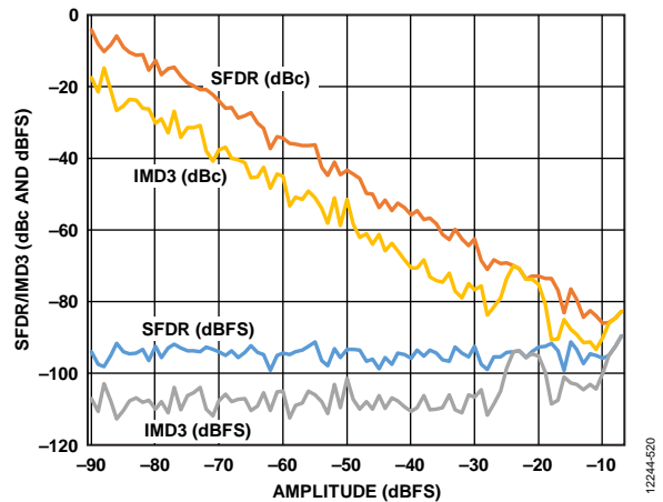
Figure 43. Two-Tone SFDR/IMD3 vs. Input Amplitude ( A_{IN} ) with f_{IN1} = 184 MHz and f_{IN2} = 187 MHz
