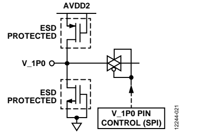
Figure 62. V_1P0 Input
