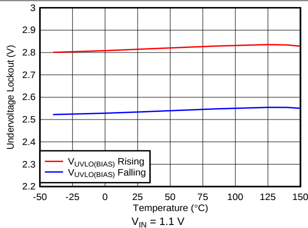
Figure 33. V_{BIAS} UVLO vs Temperature
