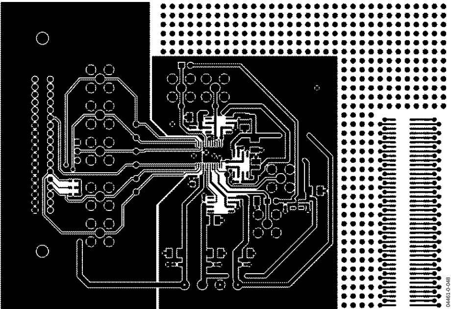
Figure 48. Component-Side Artwork
