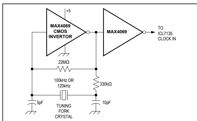
Figure 8B. Crystal Oscillator Clock Source
