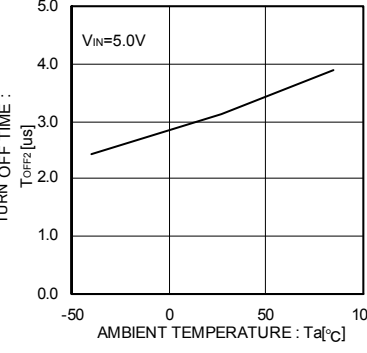
Fig.23 Output turn off time
