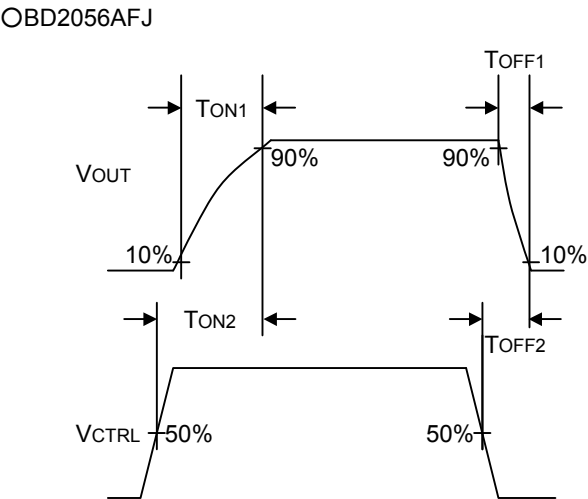
Fig.3 Timing diagram
