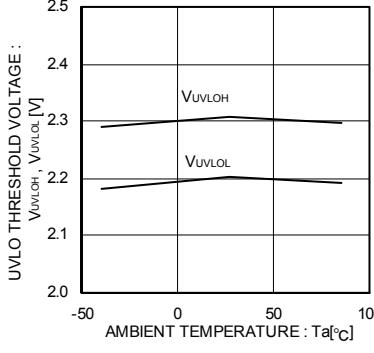
Fig.24 UVLO threshold voltage
