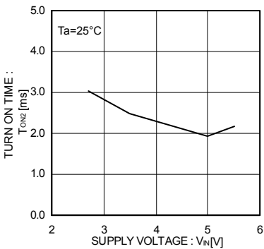
Fig.18 Output turn on time
