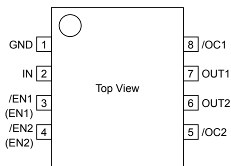
Fig.37 Pin Configuration
