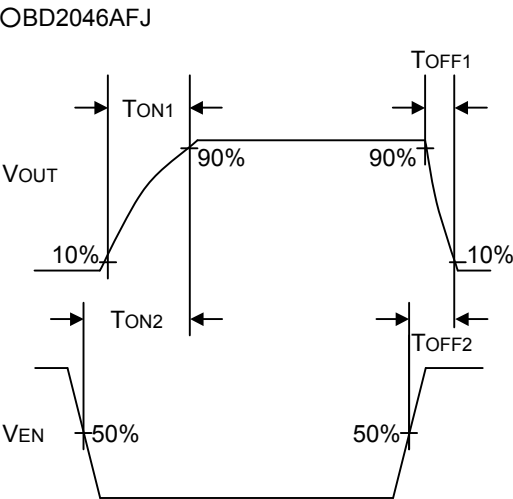
Fig.2 Timing diagram
