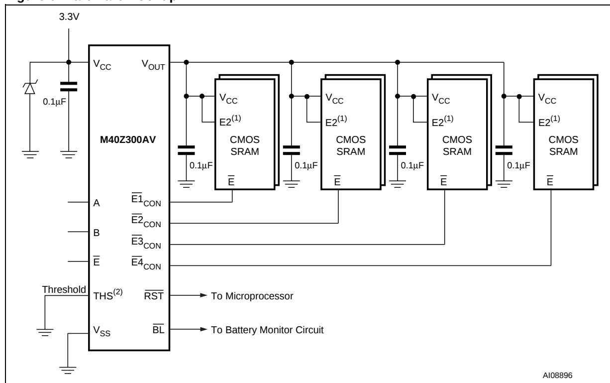
Figure 6. Hardware Hookup
