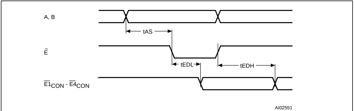
Figure 7. Address-Decode Time
