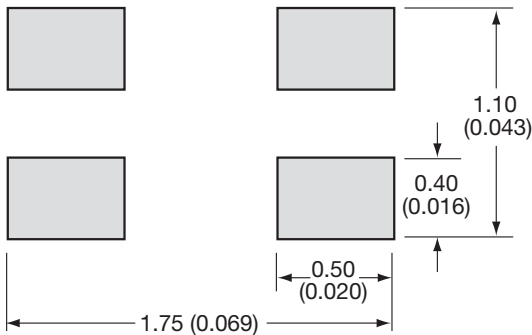
Recommended Pad Layout Dimensions mm (inches)
