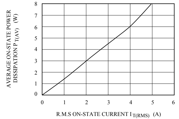
P_{T(AV)} - I_{T(RMS)}
