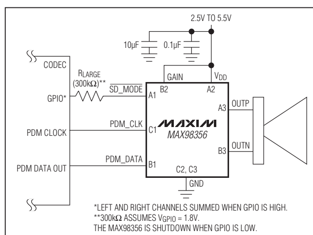
Figure 10. (Left + Right)/2 Operation with 6dB Gain
