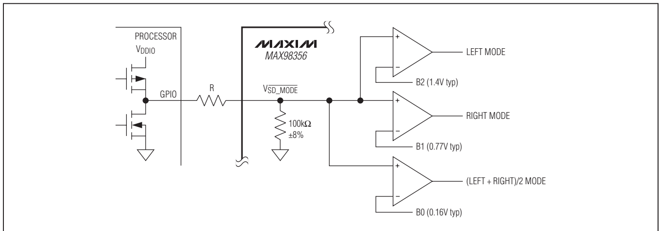
Figure 4. \overline{\text{SD\_MODE}} Resistor Connection Using Pullup/Down Driver
