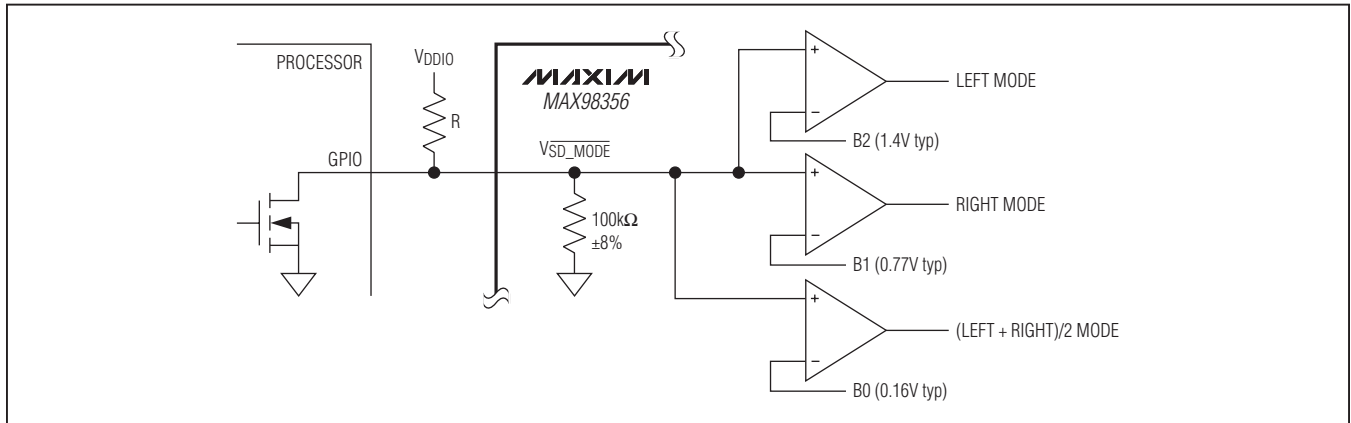
Figure 3. \overline{\text{SD\_MODE}} Resistor Connection Using Open-Drain Driver
