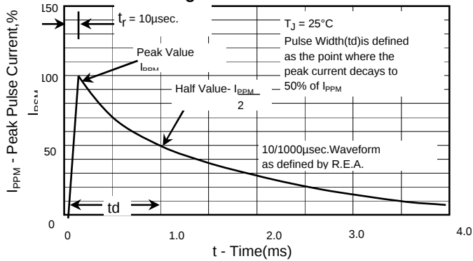
Fig. 3 - Pulse Waveform
