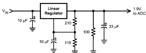
FIGURE 23. Non-Spiking Power Supply
