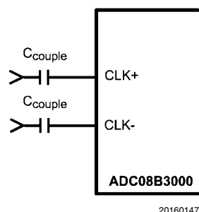
FIGURE 20. Differential Sample Clock Connection
