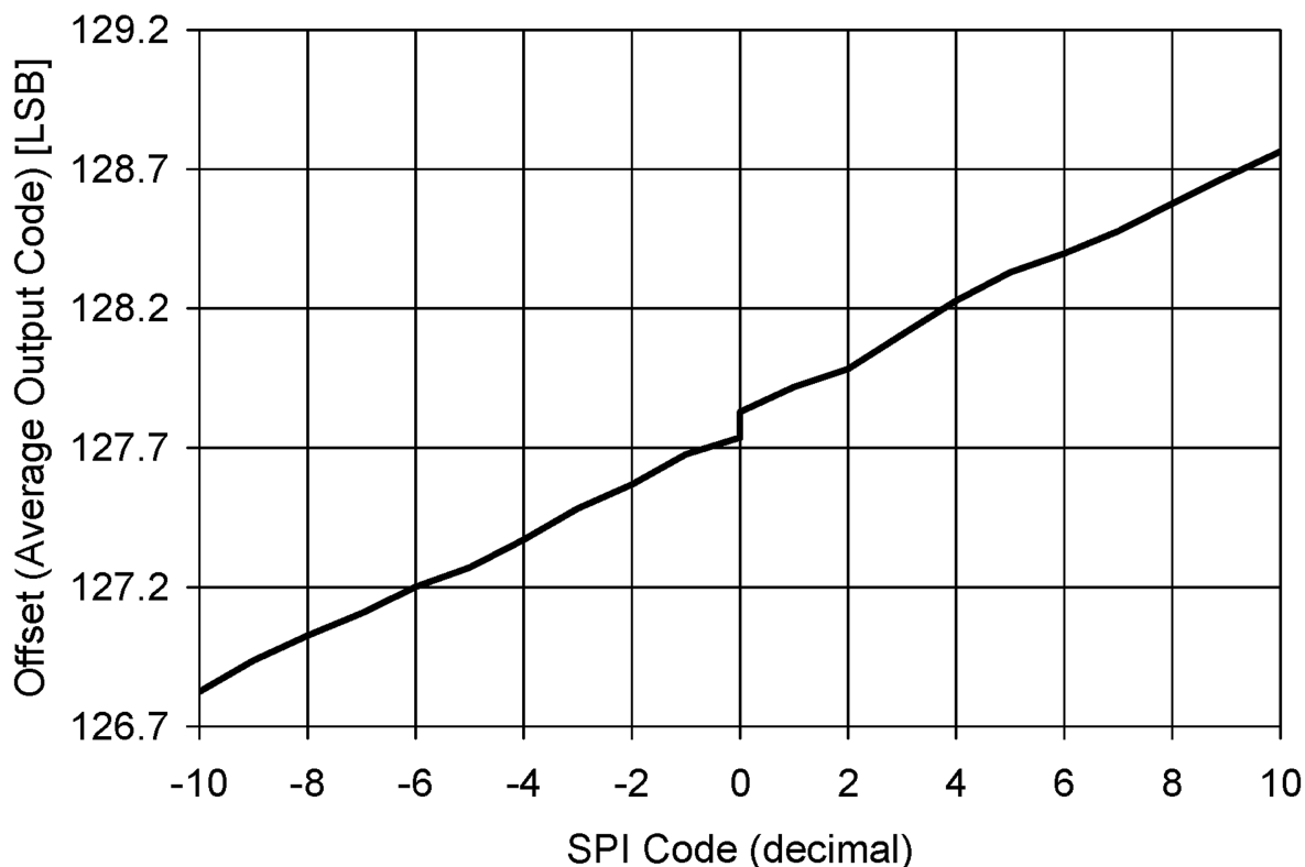
FIGURE 16. Extended Mode Offset Behavior
