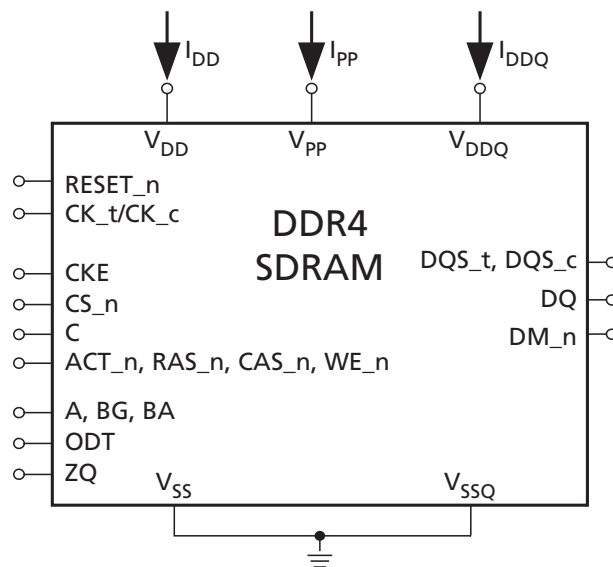
Figure 239: Measurement Setup and Test Load for I_{DDx} , I_{DDPx} , and I_{DDQx}
