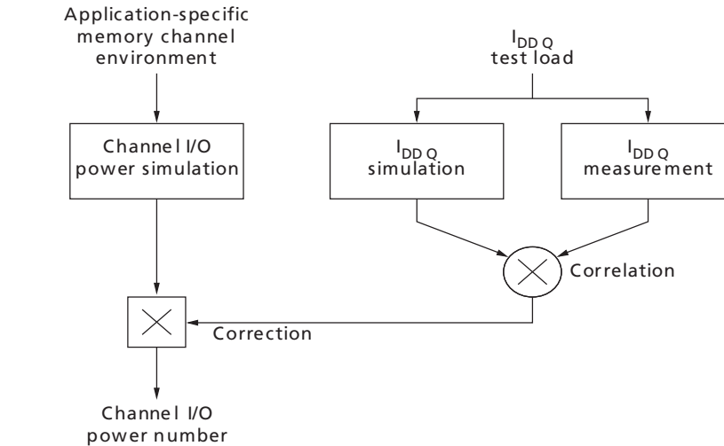
Figure 240: Correlation: Simulated Channel I/O Power to Actual Channel I/O Power
