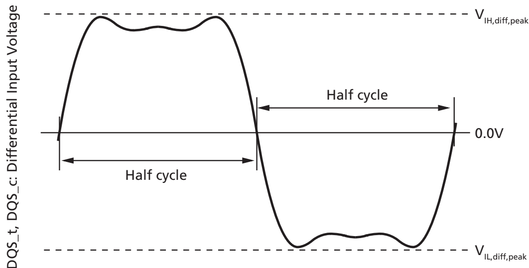
Figure 218: Differential Input Signal Definition for DQS t , DQS c
