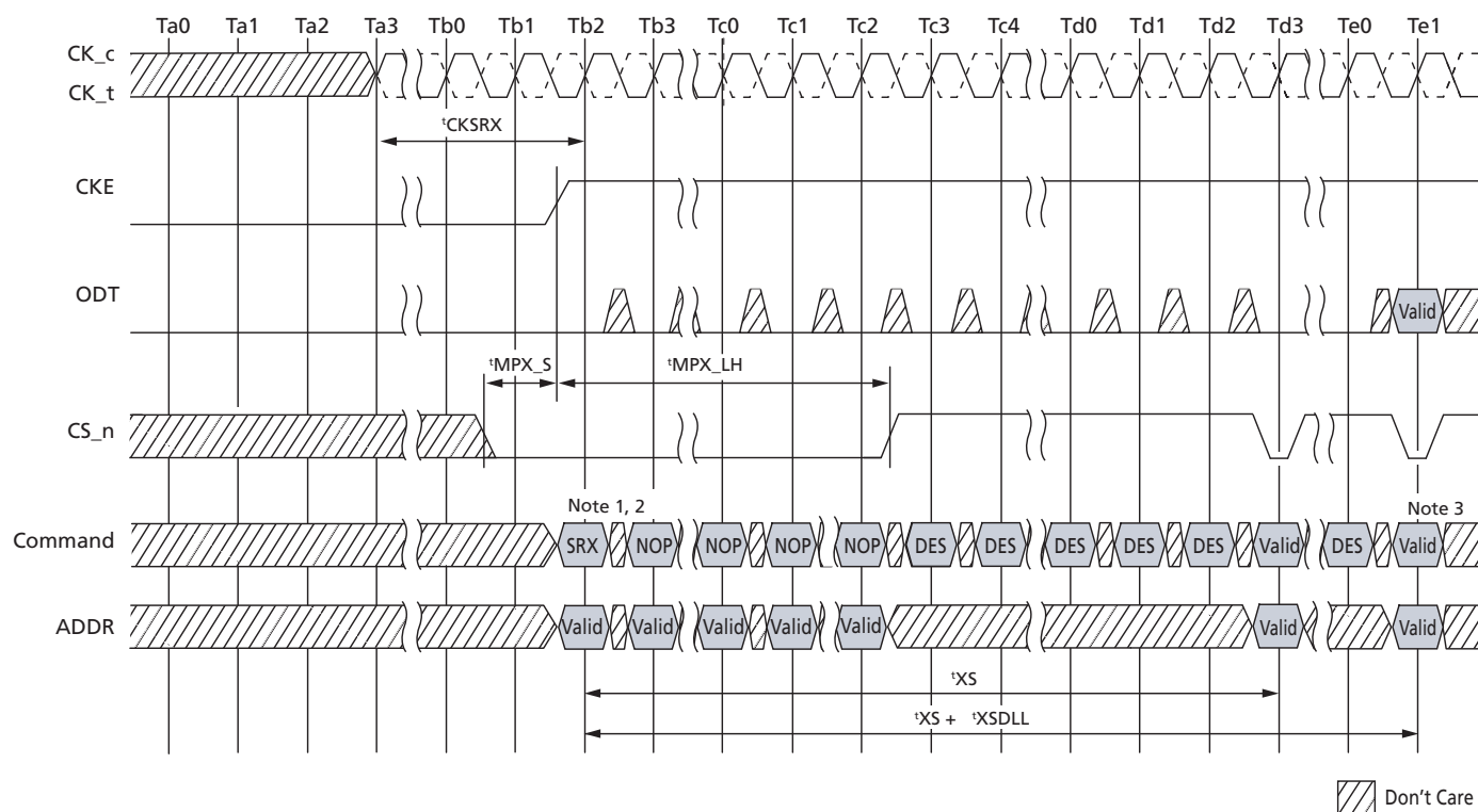
Figure 86: Self Refresh Exit with NOP Command
