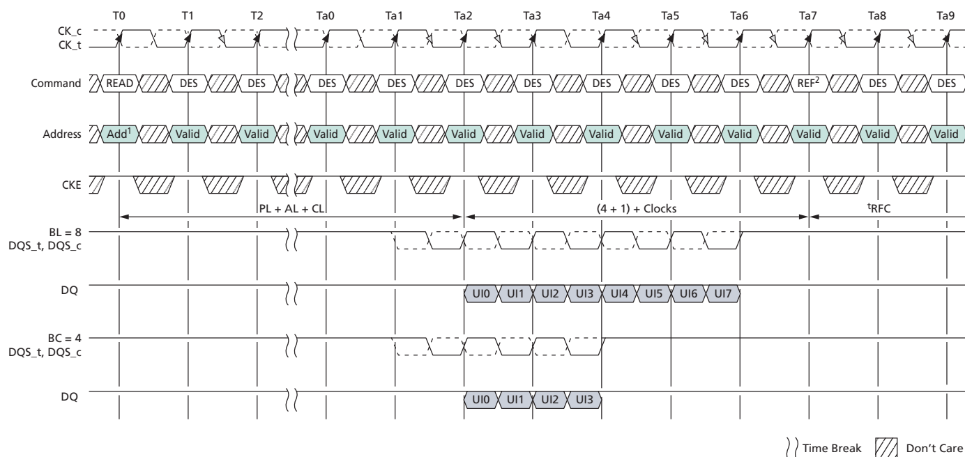
Figure 36: READ-to-REFRESH Timing
