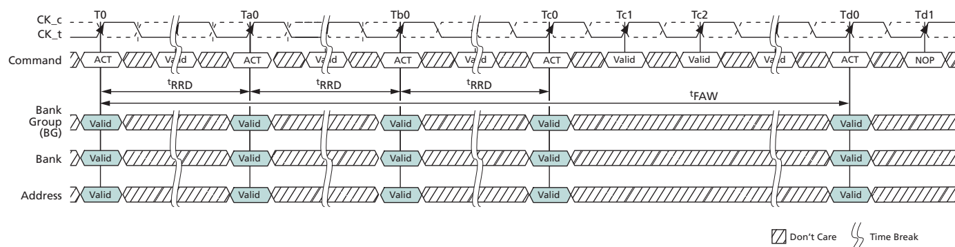
Figure 76: t_{FAW} Timing
