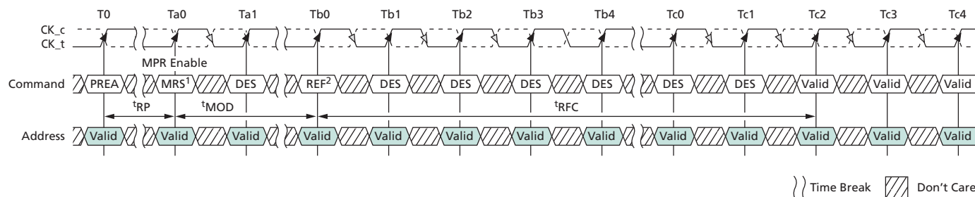
Figure 35: REFRESH Timing
