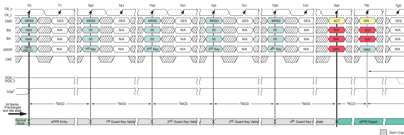
Figure 73: sPPR – Entry
