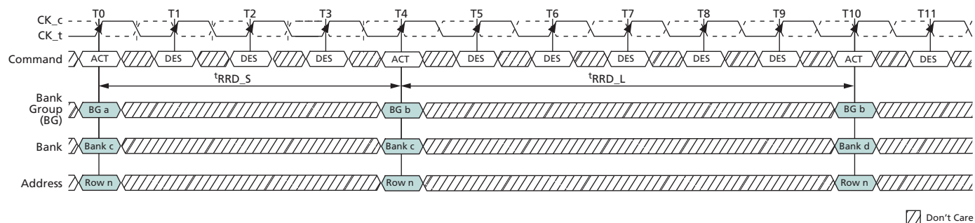
Figure 115: t_{RRD} Timing
