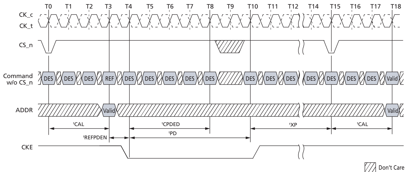
Figure 98: REFRESH Command to Power-Down Entry with CAL
