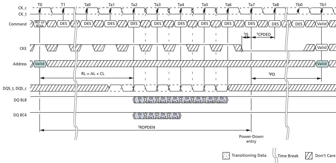
Figure 88: Power-Down Entry After Read and Read with Auto Precharge
