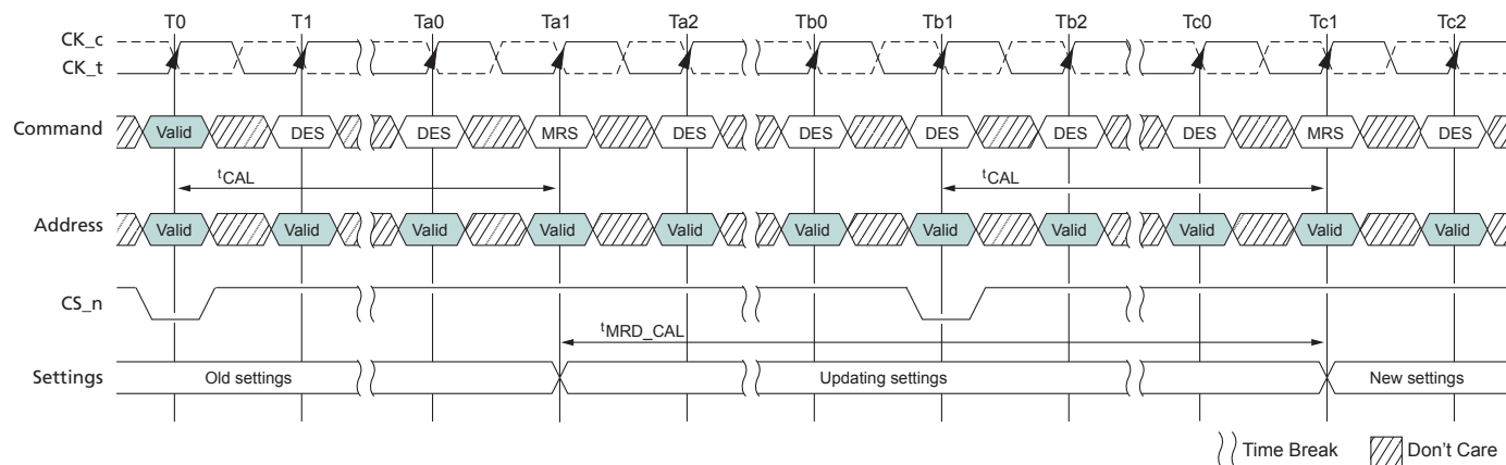
Figure 25: t_{MRD\_CAL} , Mode Register Cycle Time With CAL Enabled
