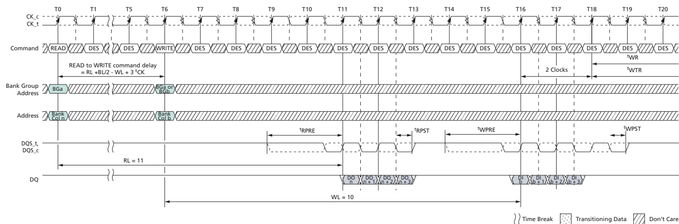
Figure 141: READ (BC4) Fixed to WRITE (BC4) Fixed with 2^t\text{CK} Preamble in Same or Different Bank Group
