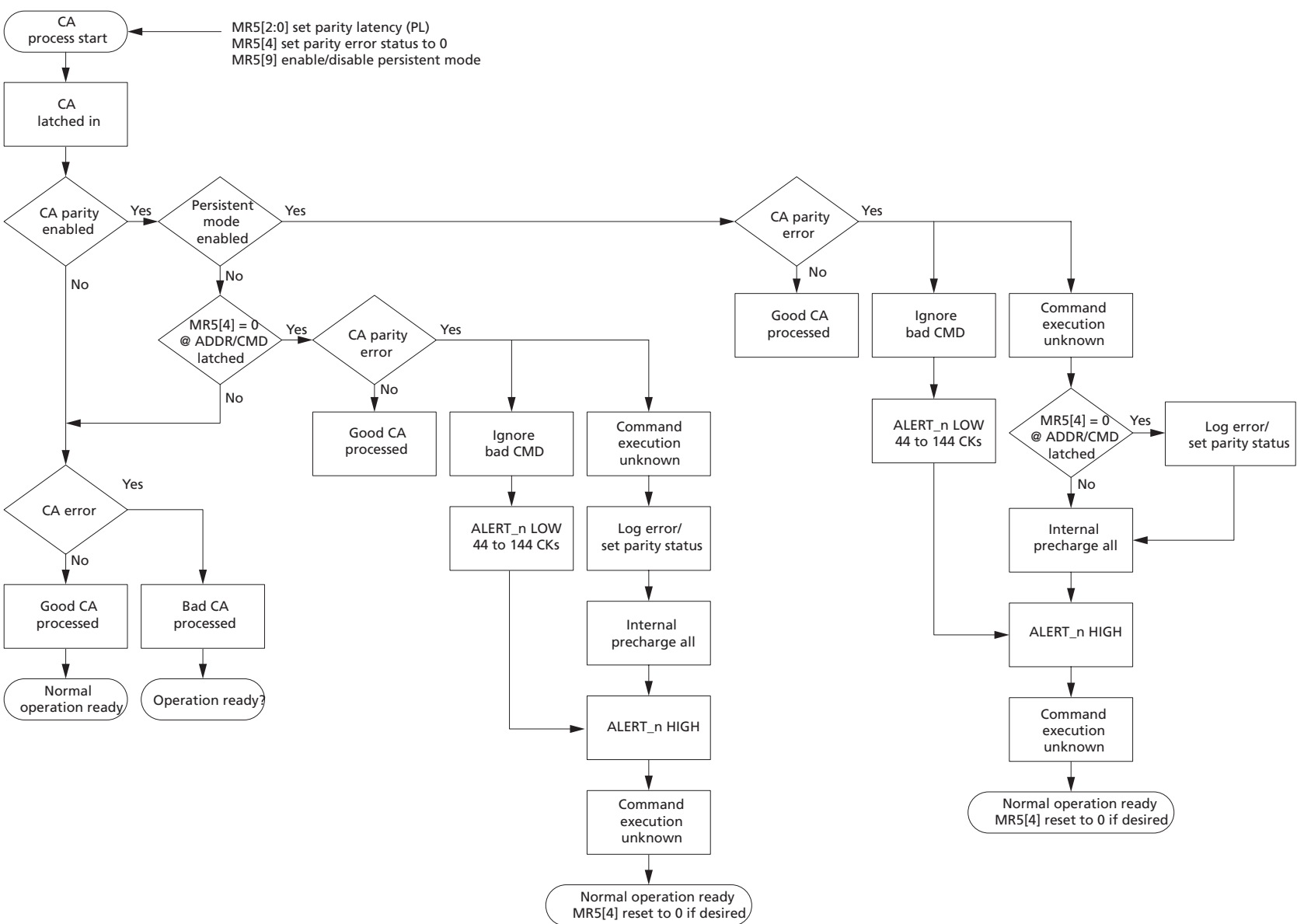
Figure 55: CA Parity Flow Diagram
