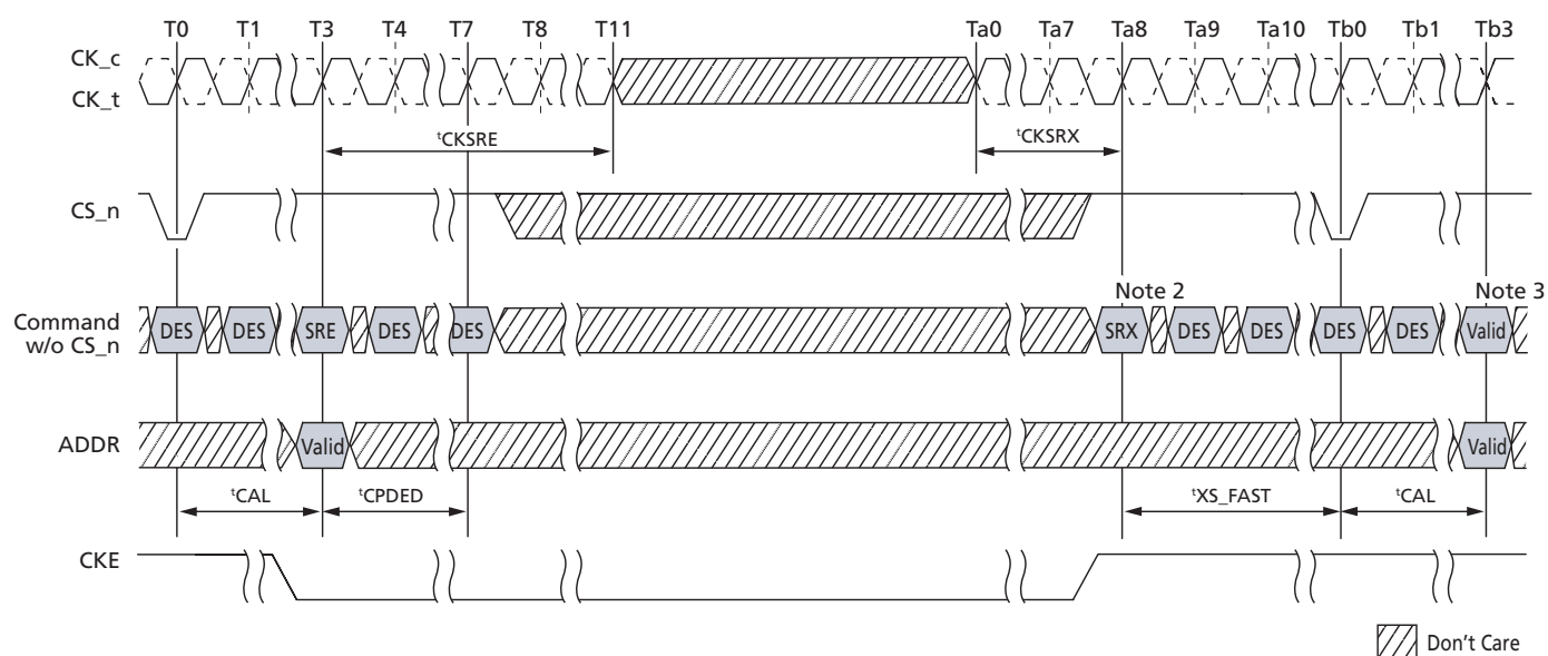
Figure 84: Self Refresh Entry/Exit Timing with CAL Mode
