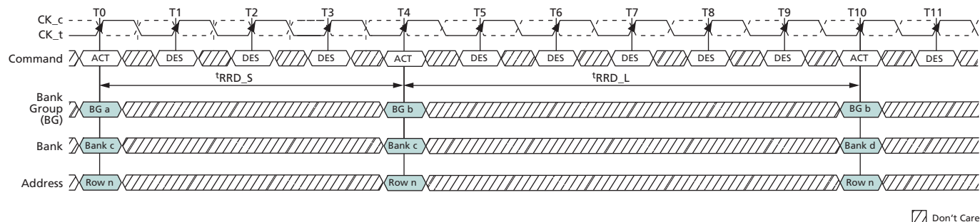
Figure 75: t_{RRD} Timing
