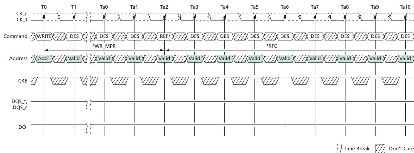
Figure 37: WRITE-to-REFRESH Timing
