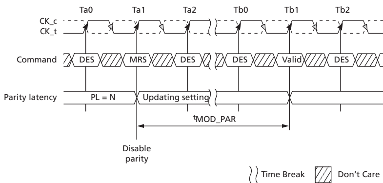
Figure 54: Parity Exit Timing Example – t_{MOD\_PAR}
