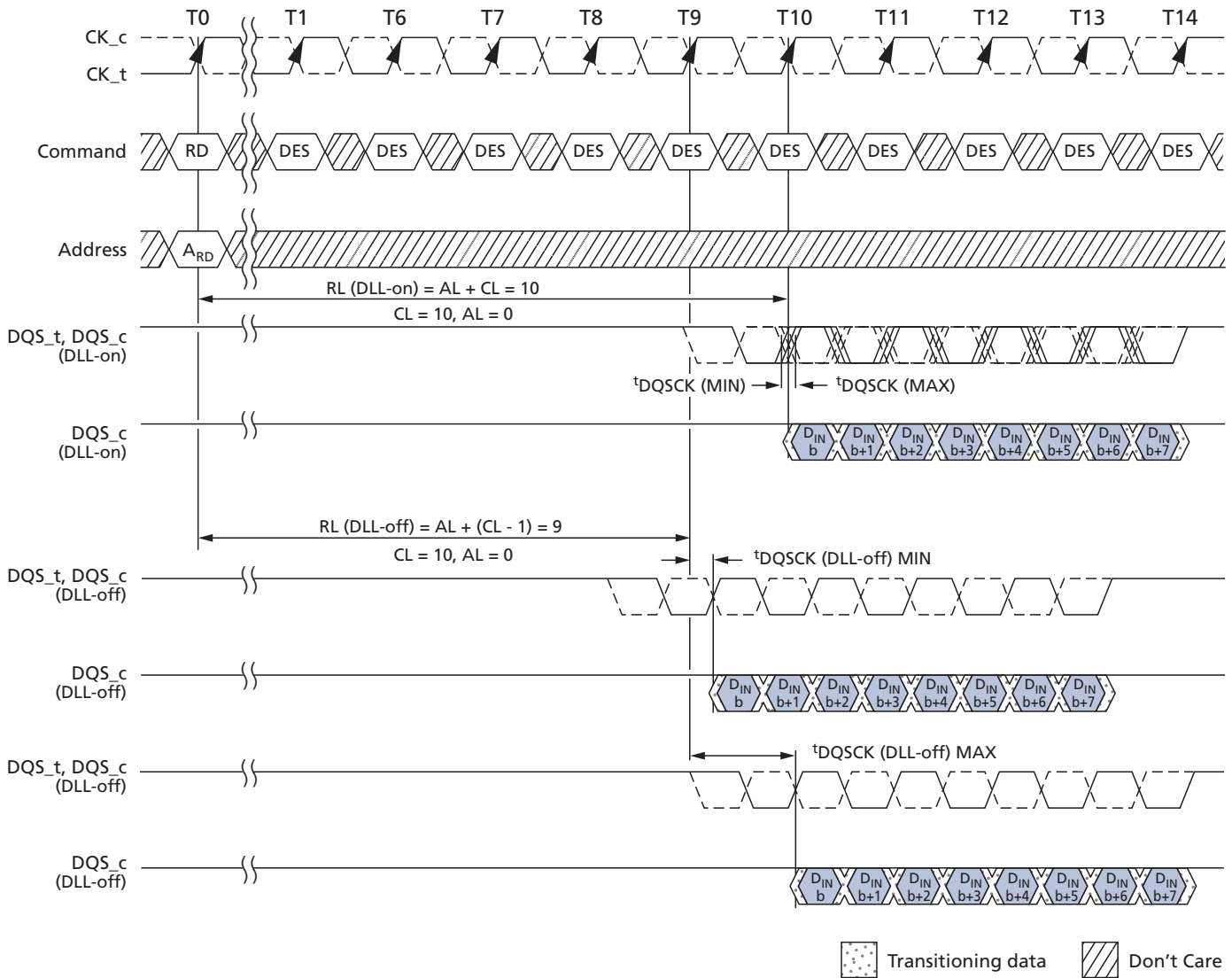
Figure 13: DLL-Off Mode Read Timing Operation
