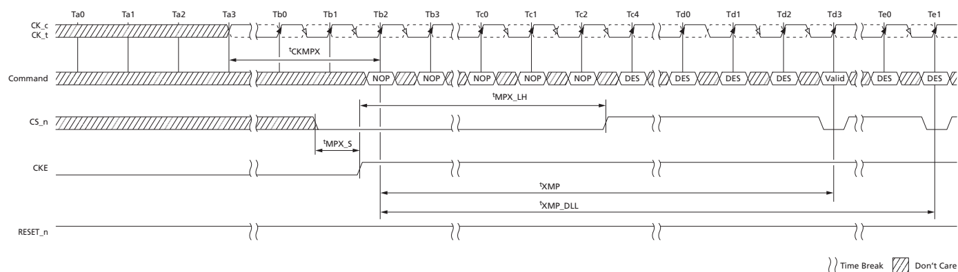
Figure 44: Maximum Power-Saving Mode Exit
