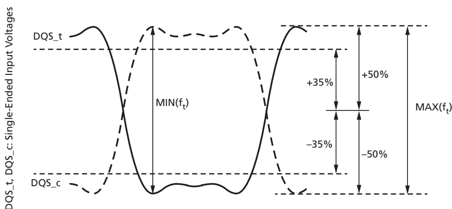
Figure 219: DQS_t, DQS_c Input Peak Voltage Calculation and Range of Exempt non-Monotonic Signaling
