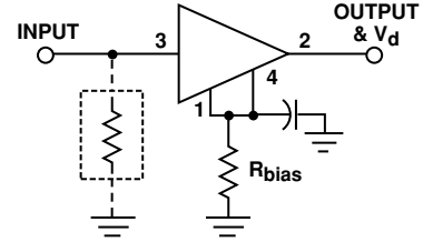
Figure 4. Source Resistor Bias.
