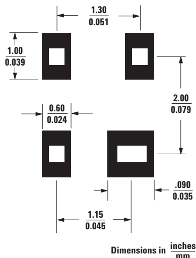
Figure 10. Recommended PCB Pad Layout for Agilent's SC70 4L/SOT-343 Products.
