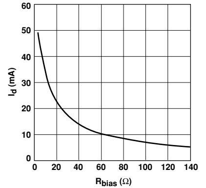
Figure 5. Device Current vs. R_{bias} .
