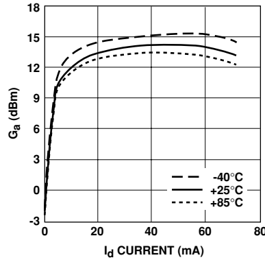
Figure 16. Associated Gain (Fmin) vs. Current and Temperature.
