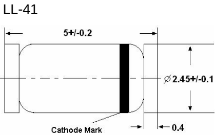
Glass case MELF Dimensions in mm
