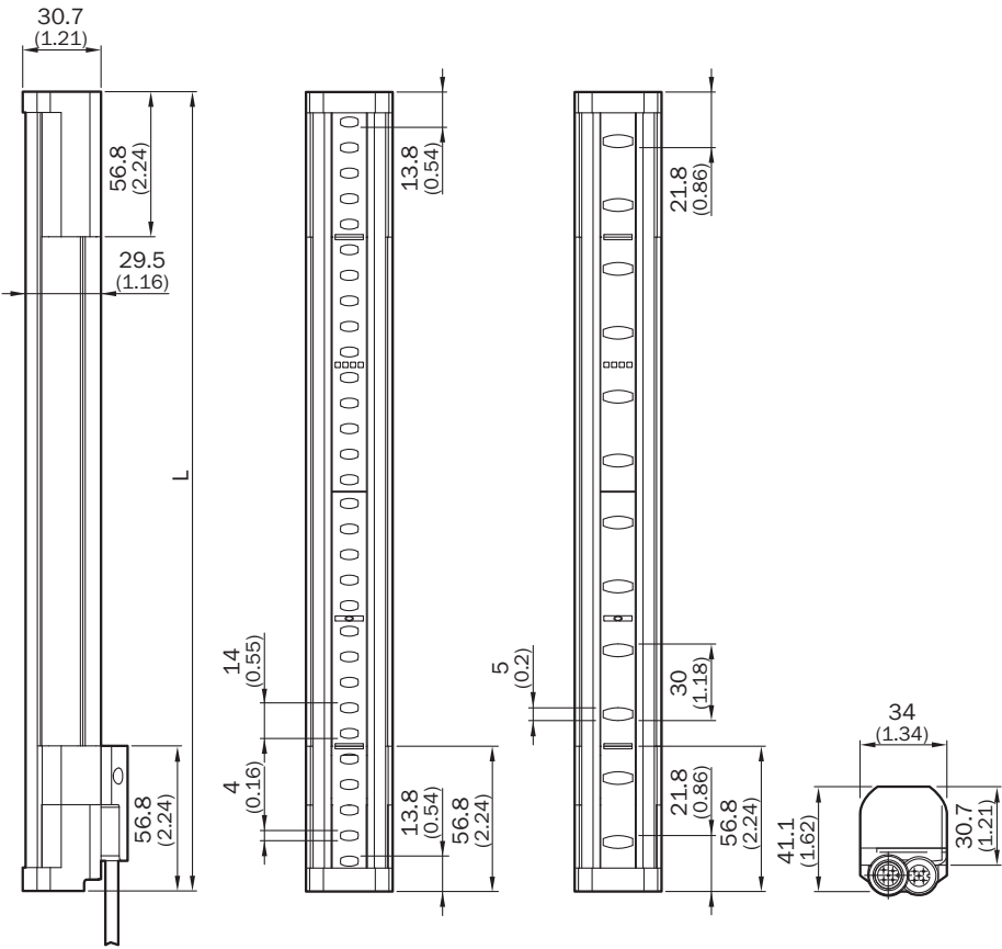
Dimensional drawing (Dimensions in mm (inch))
