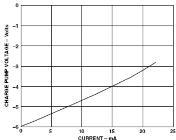
Figure 3. Charge Pump Voltage vs. Current
