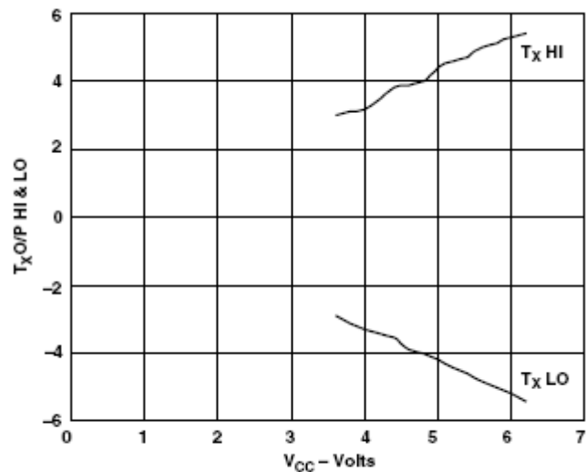
Figure 6. Tx Output Voltage vs. Supply
