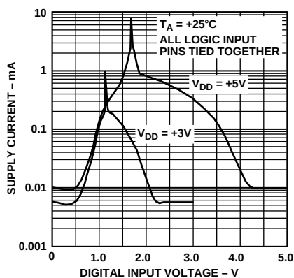
Figure 26. Supply Current vs. Input Logic Voltage
