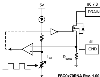
Figure 16. Soft-Start Function
