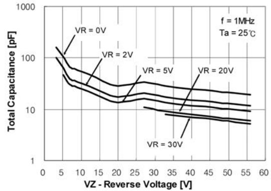
Figure 2. Total Capacitance
