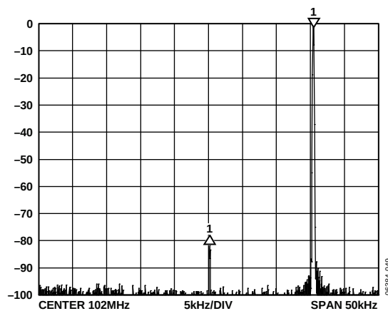
Figure 8. Narrow-Band View of Figure 5 (with Carrier and Lower Sideband Suppression)
