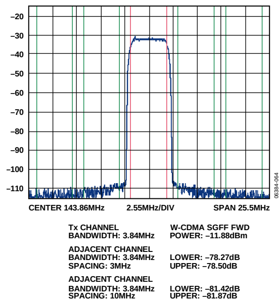
Figure 24. Typical ACLR for Wideband CDMA
