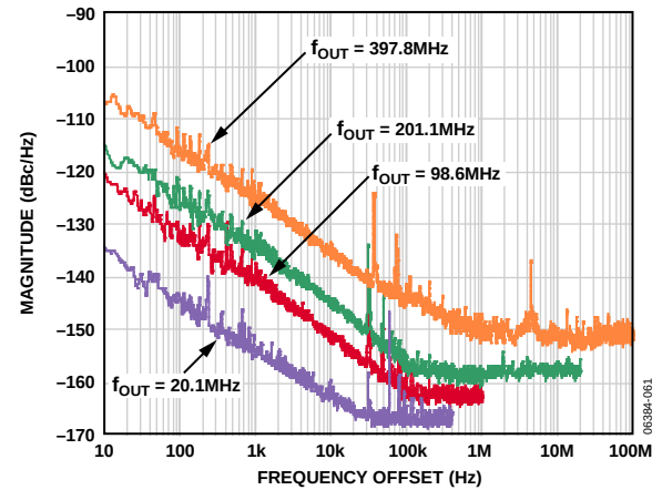
Figure 20. Residual Phase Noise, System Clock = 1 GHz
