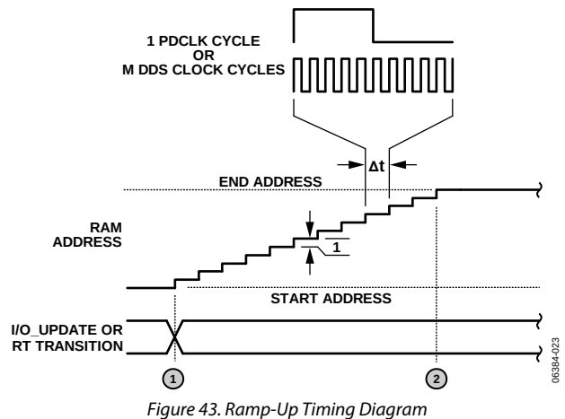
Figure 43. Ramp-Up Timing Diagram
