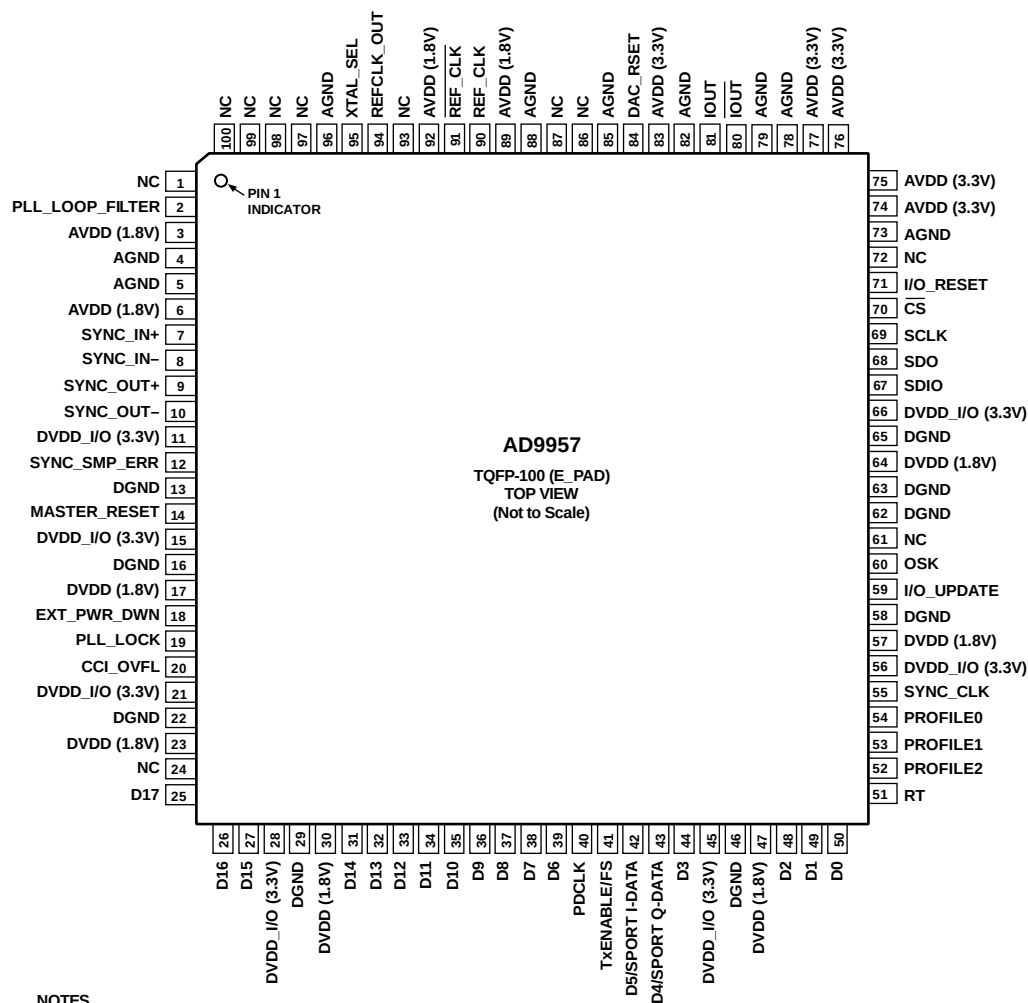
Figure 4. Pin Configuration
