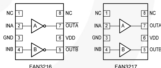
Figure 1. Pin Configurations
