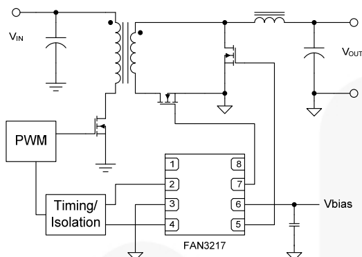
Figure 34. Forward Converter with Synchronous Rectification
