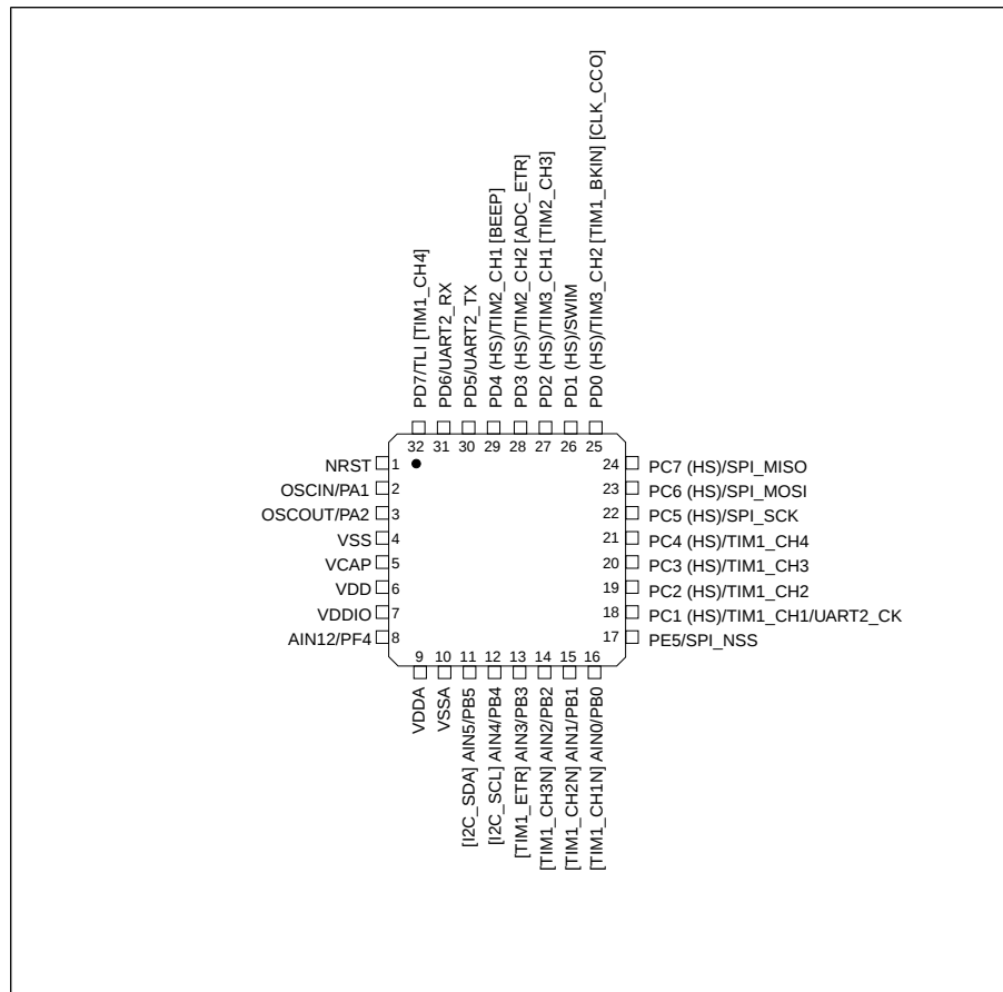
Figure 5: LQFP/UFQFPN 32-pin pinout
