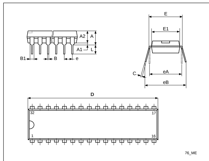
Figure 51: 32-lead shrink plastic DIP (400 ml) package
