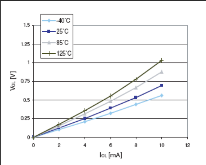
Figure 28: Typ. V_{OL} @ V_{DD} = 3.3\text{ V} (standard ports)
