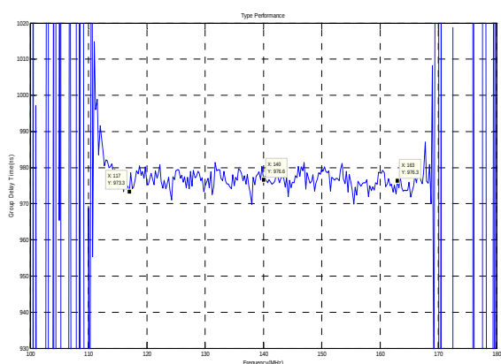
Group Delay Variation( f_0 \pm 23\text{MHz} )
