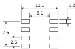
SUGGESTED PAD LAYOUT
