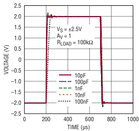
Large-Signal Response
