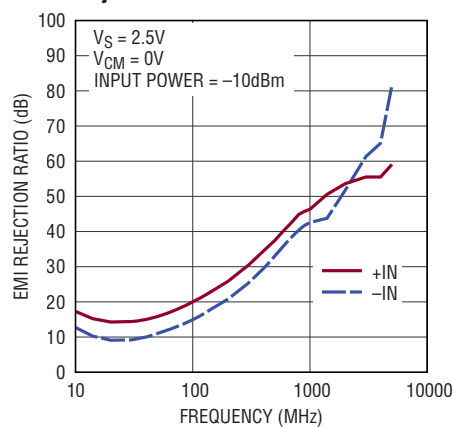
Electromagnetic Interference Rejection Ratio
