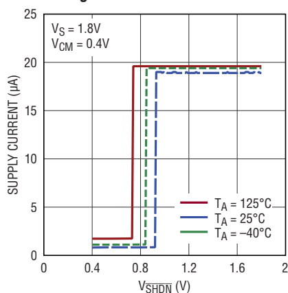
Supply Current vs \overline{SHDN} Pin Voltage
